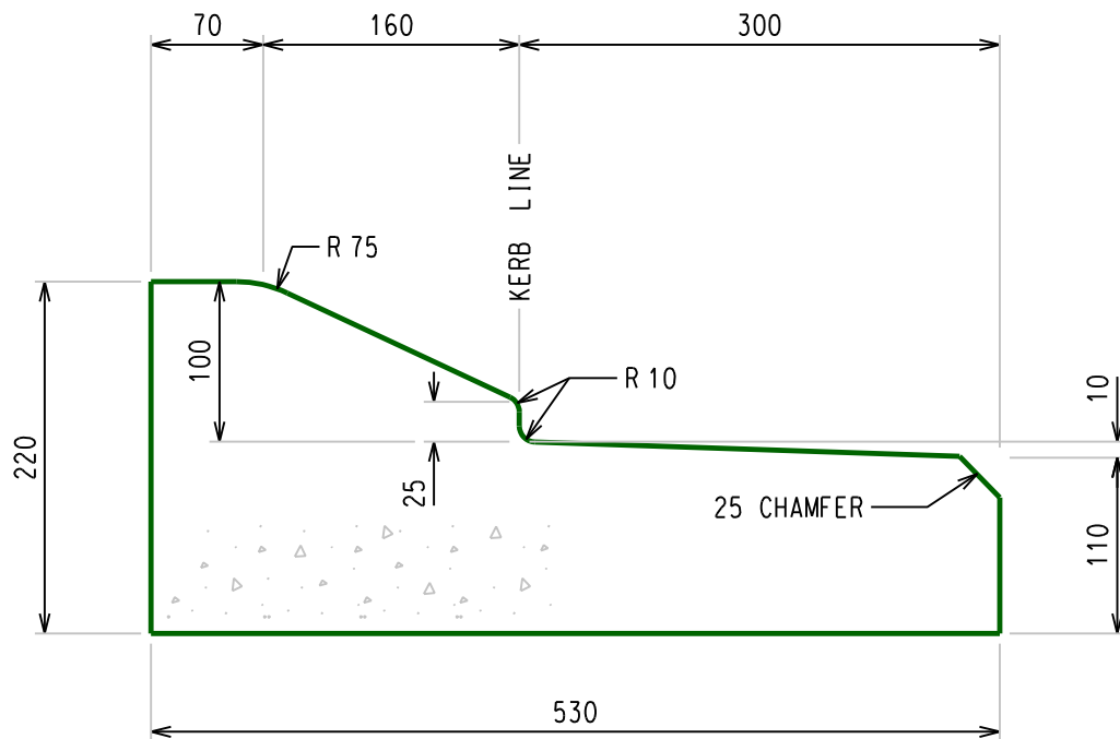
KERB and TRAY
