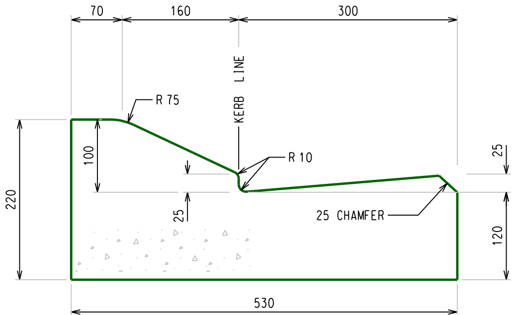
KERB and CHANNEL
